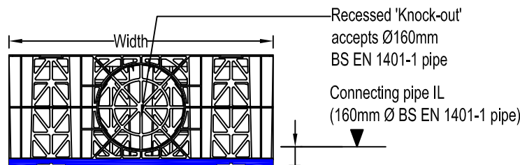
END ELEVATION Scale 1:10
