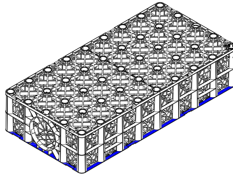
ISOMETRIC VIEW Scale 1:10
